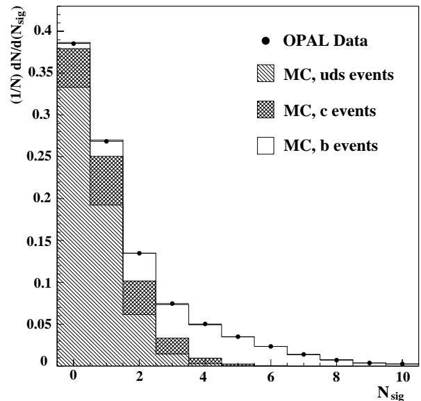
Fig. 1. Distribution of number of tracks per event ( N_{sig} ) with b/\sigma_b > 2.5 . The points are data and the solid histogram is Monte Carlo. The Monte Carlo is also shown decomposed into contributions from uds, c and b quark events
