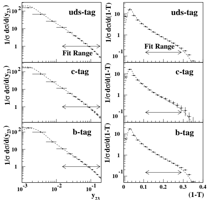
Fig. 4. The points with error bars are the distributions of y_{23} and 1-T measured in three flavour-tagged event samples (uds-tag, c-tag and b-tag) corrected to the hadron level. The curves show the result of simultaneous fits of \mathcal{O}(\alpha_s^2) calculations to the distributions measured in each flavour-tagged event sample. The renormalization scale x_\mu was fixed equal to one. The fit range for each distribution is indicated by the arrows
