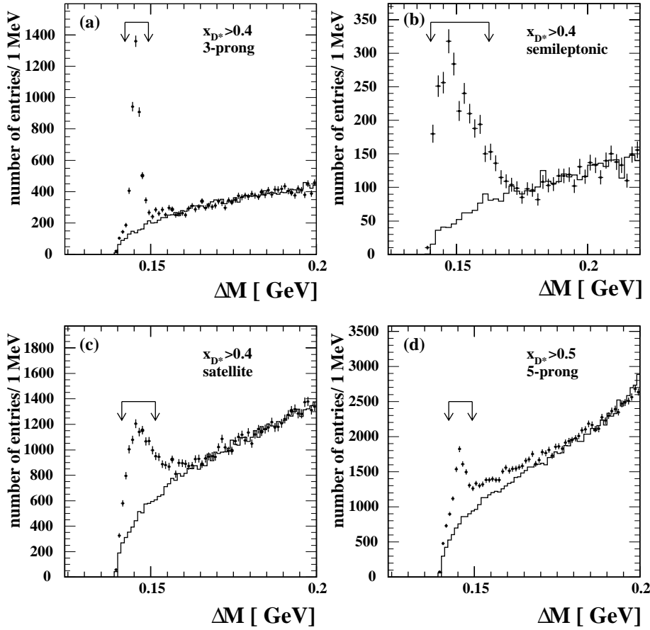
Fig. 2a–d. Distribution of the mass difference \Delta M for four different D^{*+} decay channels: a 3-prong decay mode, b the two semileptonic modes combined, c the satellite decay mode, and d the 5-prong decay mode. The arrows indicate the selected signal regions. The points with error bars are the signal candidates and the solid histograms are the background estimator distributions
