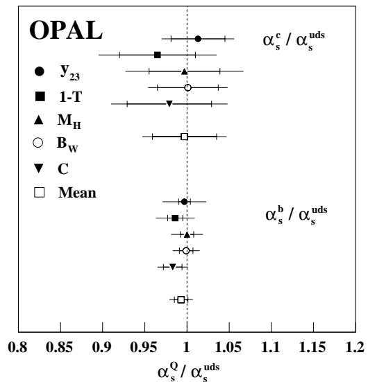
Fig. 7. The ratios \alpha_s^c/\alpha_s^{\text{uds}} and \alpha_s^b/\alpha_s^{\text{uds}} determined for each of the event shapes studied. The weighted mean of the results derived for the five event shape observables is also shown. The inner error bar represents the statistical error while the full error bar represents the statistical error and the systematic error added in quadrature
