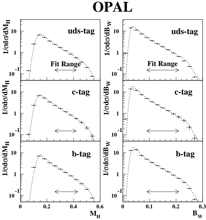
Fig. 5. The points with error bars are the distributions of M_H and B_W measured in three flavour-tagged event samples (uds-tag, c-tag and b-tag) corrected to the hadron level. The curves show the result of simultaneous fits of \mathcal{O}(\alpha_s^2) calculations to the distributions measured in each flavour-tagged event sample. The renormalization scale x_\mu was fixed equal to one. The fit range for each distribution is indicated by the arrows
