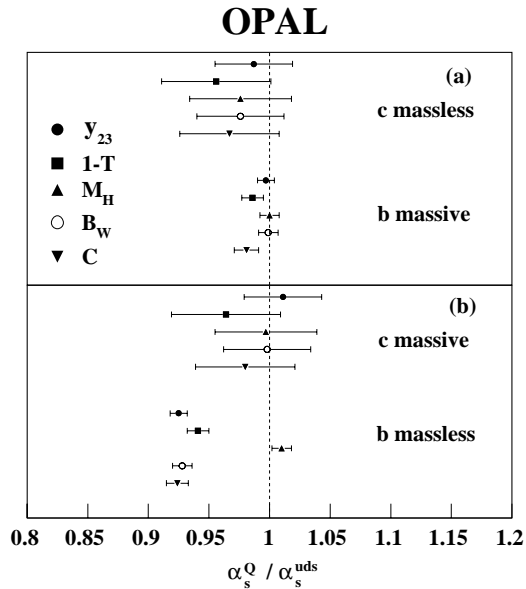
Fig. 8a,b. The ratios \alpha_s^c/\alpha_s^{uds} and \alpha_s^b/\alpha_s^{uds} determined in two different ways: a where the uds and c quarks were treated as if massless and the b quark was considered to be massive and b where the uds and b quark were treated as massless and the c quark was considered massive. The errors shown are statistical only
