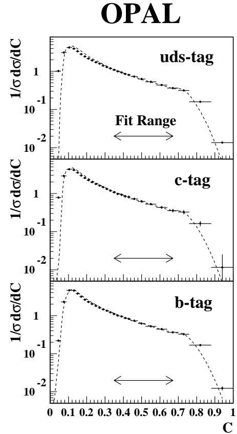
Fig. 6. The points with error bars are the distribution of the C parameter measured in three flavour-tagged event samples (uds-tag, c-tag and b-tag) corrected to the hadron level. The curves show the result of simultaneous fits of \mathcal{O}(\alpha_s^2) calculations to the distributions measured in each flavour-tagged event sample. The renormalization scale x_\mu was fixed equal to one. The fit range for each distribution is indicated by the arrows
