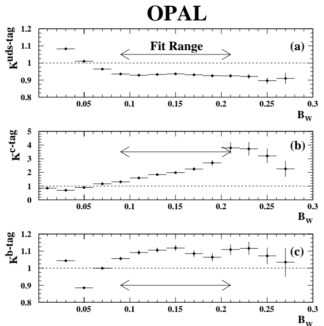
Fig. 3a–c. Bin-by-bin correction factors applied to the distribution of B_W for a the uds-tag event sample, b the c-tag event sample and c the b-tag event sample. The fit range for this observable (see Sect. 7) is indicated by the arrow on each figure
